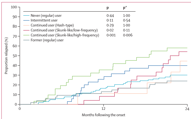
Figure: Kaplan-Meier curves of cannabis use pattern and time to relapse p values are estimated from the log-rank tests to compare the different groups (reference group is the former [regular] user group). *Bonferroni-corrected significance level.
